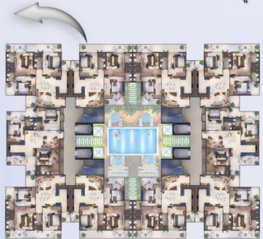
TOWER PLAN 2ND TO 13TH FLOOR
